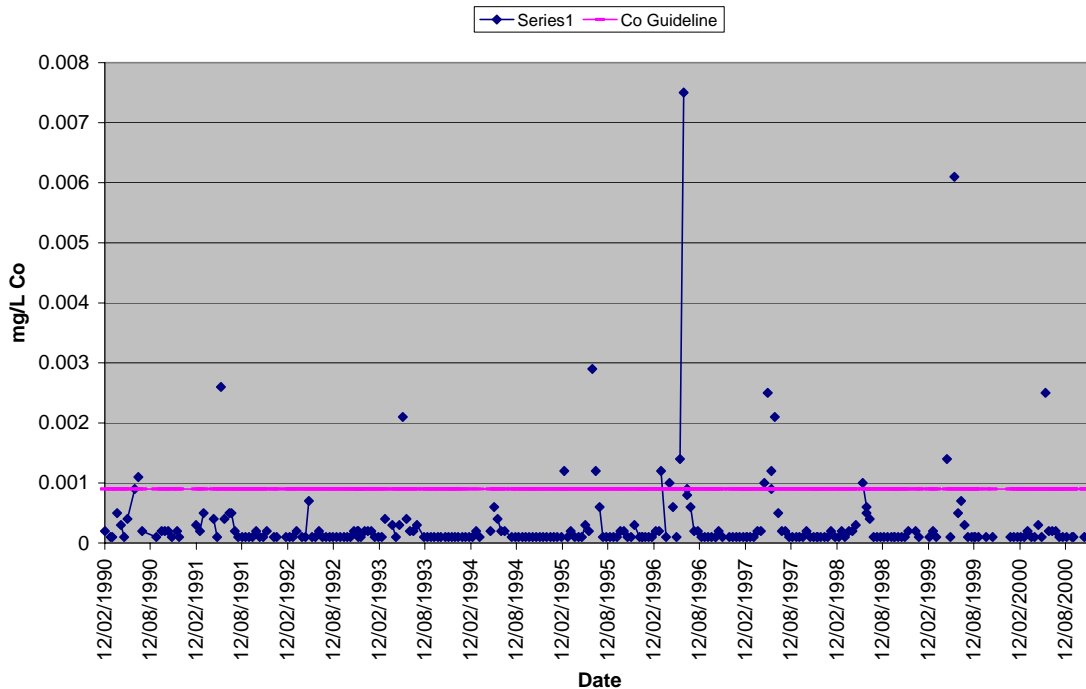
Figure 12 Elk River at Highway 93 - Total Cobalt
