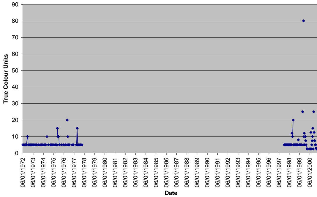
Figure 14 Elk River at Highway 93 - True Colour
