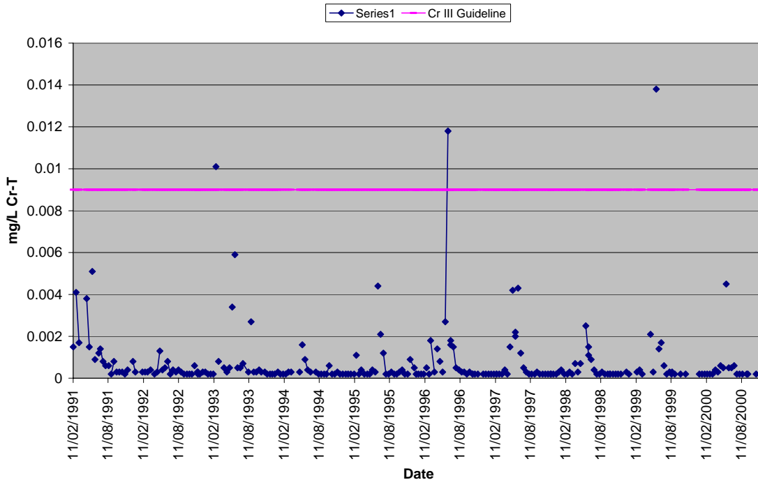
Figure 11 Elk River at Highway 93 - Total Chromium
