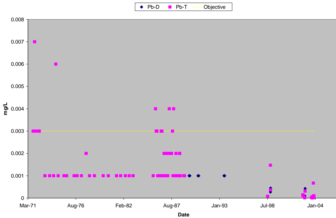
Figure 10 Lead
