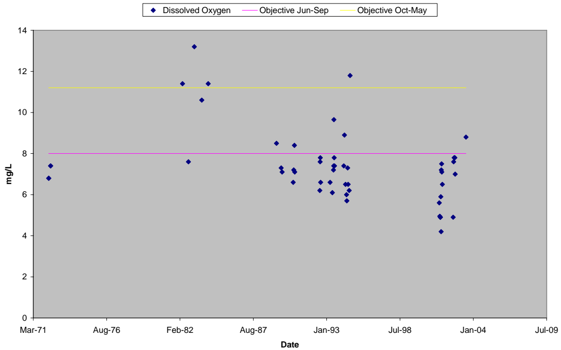
Figure 14 Oxygen, Dissolved
