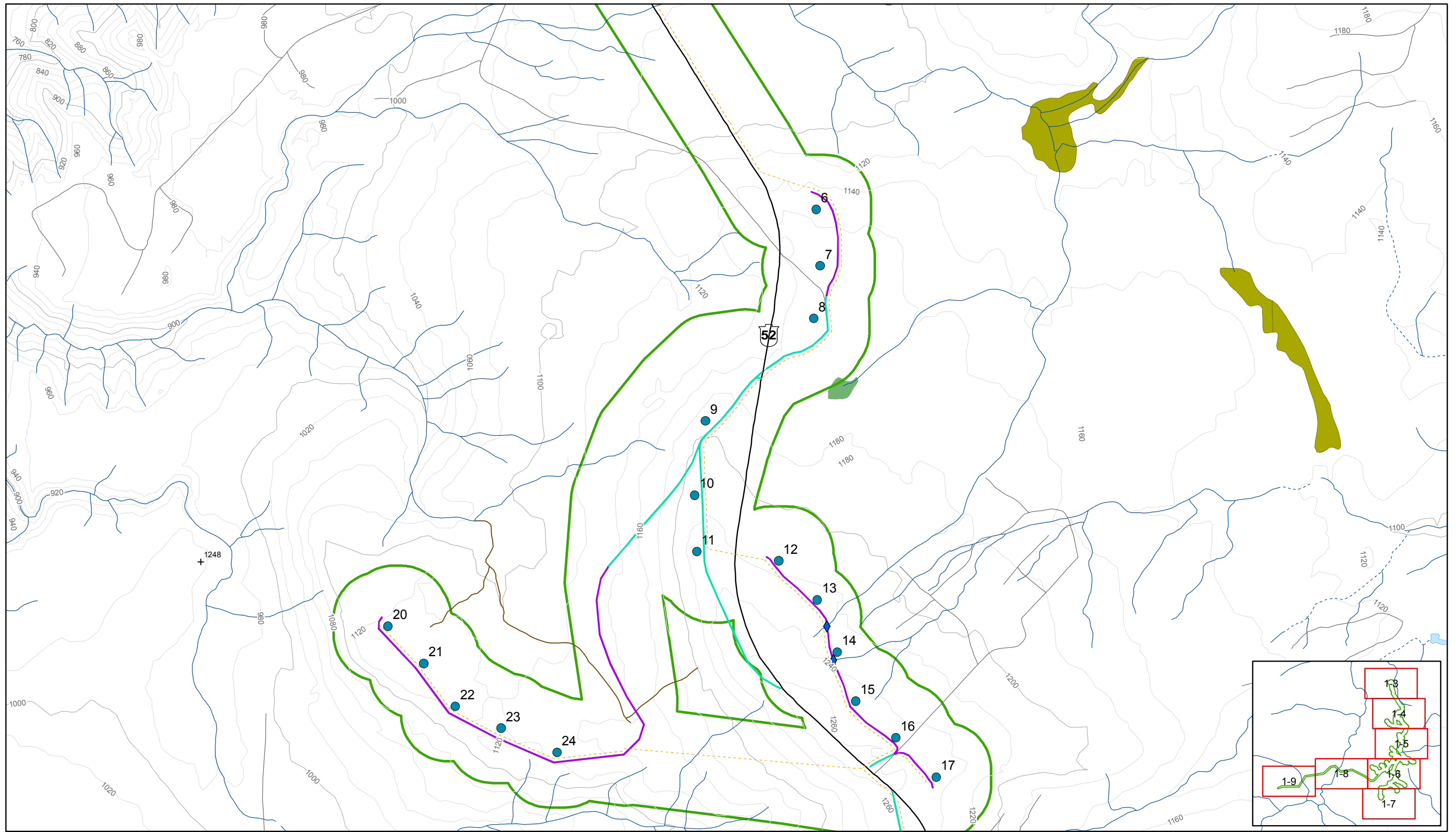
Figure 1-4 Quality Wind Project Area and Preferred Layout Quality Wind Project Environmental Assessment Application Report
