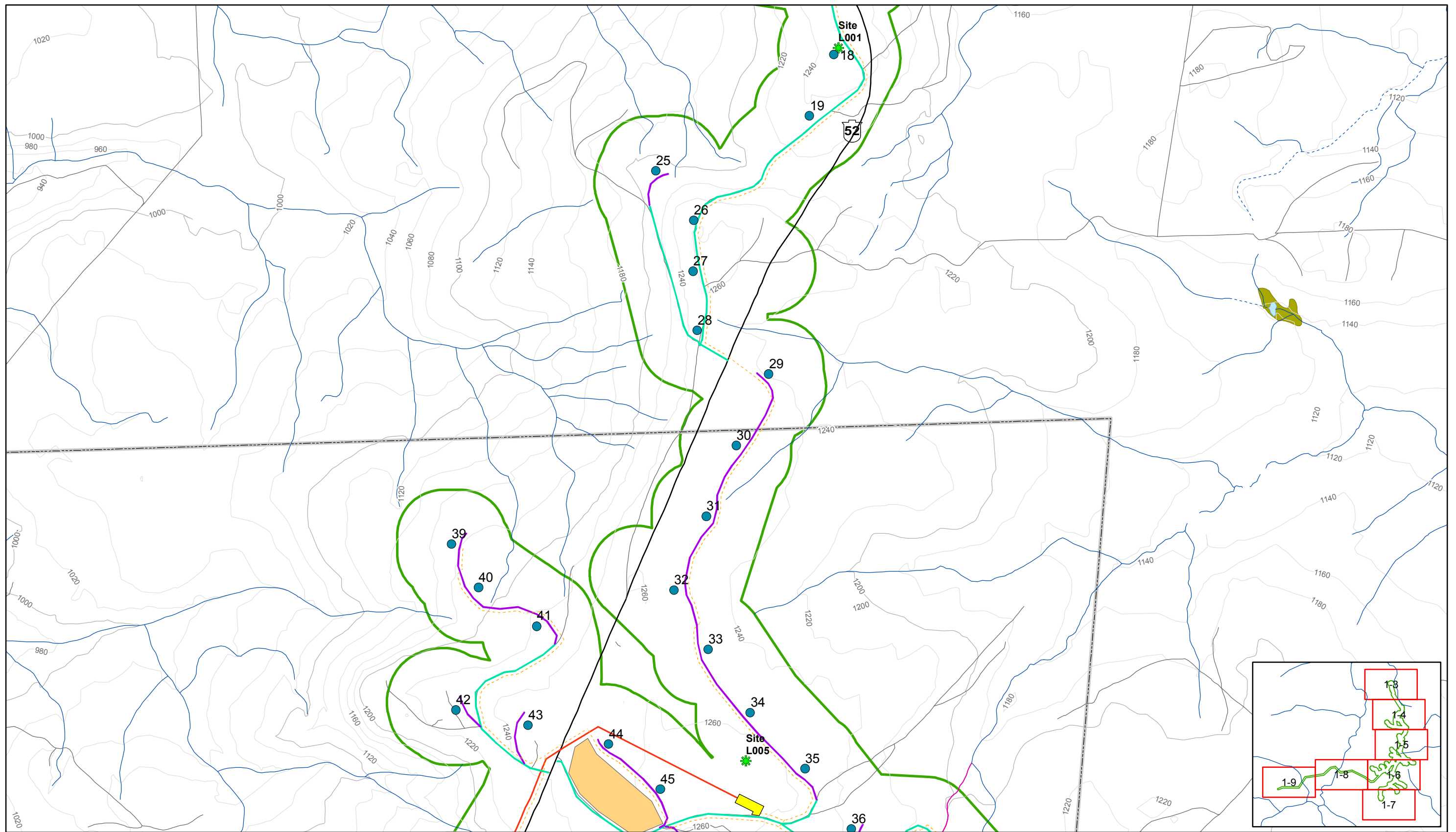
Figure 1-5 Quality Wind Project Area and Preferred Layout Quality Wind Project Environmental Assessment Application Report
