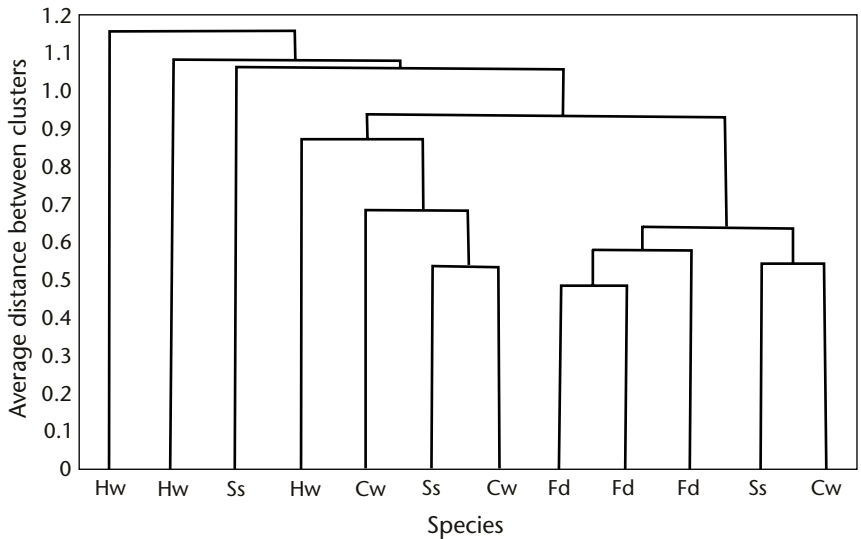
FIGURE 2 Tree diagram resulting from average linkage cluster analysis showing similarity of oribatid mite communities under three stands each of western hemlock (Hw), Sitka spruce (Ss), Douglas-fir (Fd), and western redcedar (Cw).
