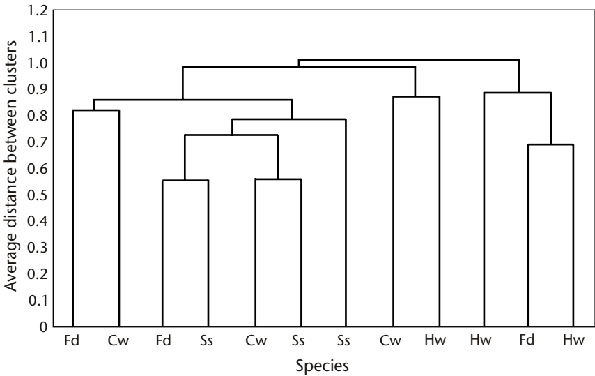
FIGURE 3 Tree diagram resulting from average linkage cluster analysis showing similarity of collembolan communities under three stands each of western hemlock (Hw), Sitka spruce (Ss), Douglas-fir (Fd), and western redcedar (Cw).
