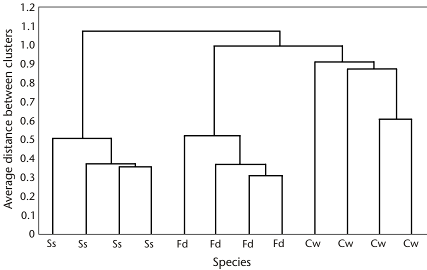
FIGURE 1 Tree diagram resulting from average linkage cluster analysis showing similarity of mushroom communities under four stands each of Sitka spruce (Ss), Douglas-fir (Fd), and western redcedar (Cw).
